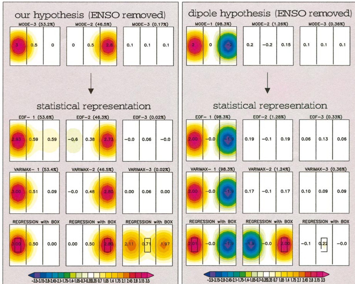
FIG. 2. As in Fig. 1, but the ENSO response mode has been removed from both hypotheses.
