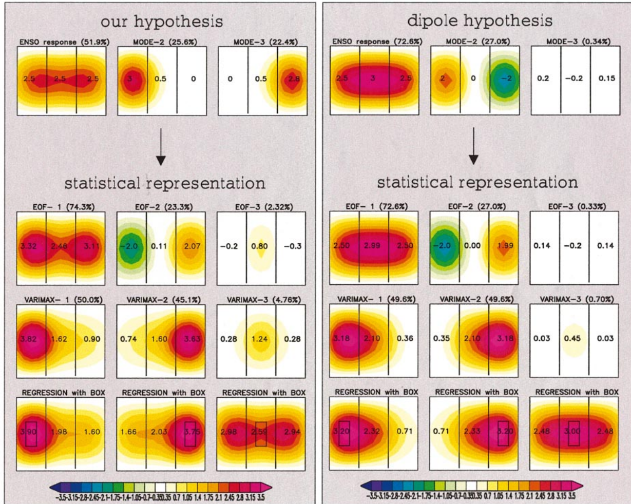
FIG. 1. The hypothetical modes and their statistical representations by EOFs, varimax patterns, and regressions of box-averaged SST in an artificial three-dimensional domain are shown for two different hypotheses. The amplitudes are in arbitrary units.
